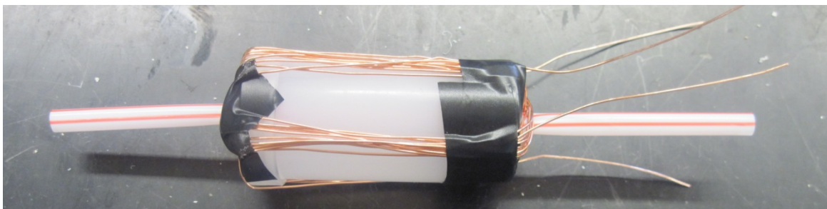
Figure 7: Step 7 – Completed motor coils.
