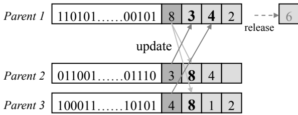
Figure 2.3 Update of tabu list
