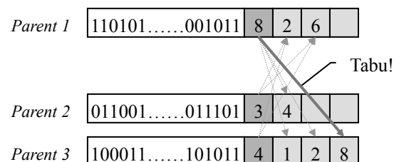
Figure 2.2 Tabu checking procedures
