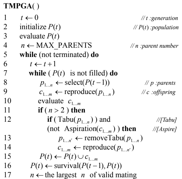
Figure 2.4 The algorithm TMPGA
