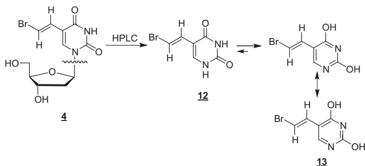
Scheme 5. Proposed resonance stabilization leading to cleavage
