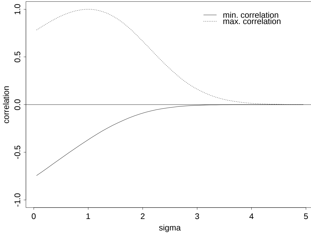
Figure 2: Maximum and minimum attainable correlations for lognormal risks X_1 and X , where \log(X_1) is standard normal and \log(X) has mean zero and variance \sigma .
