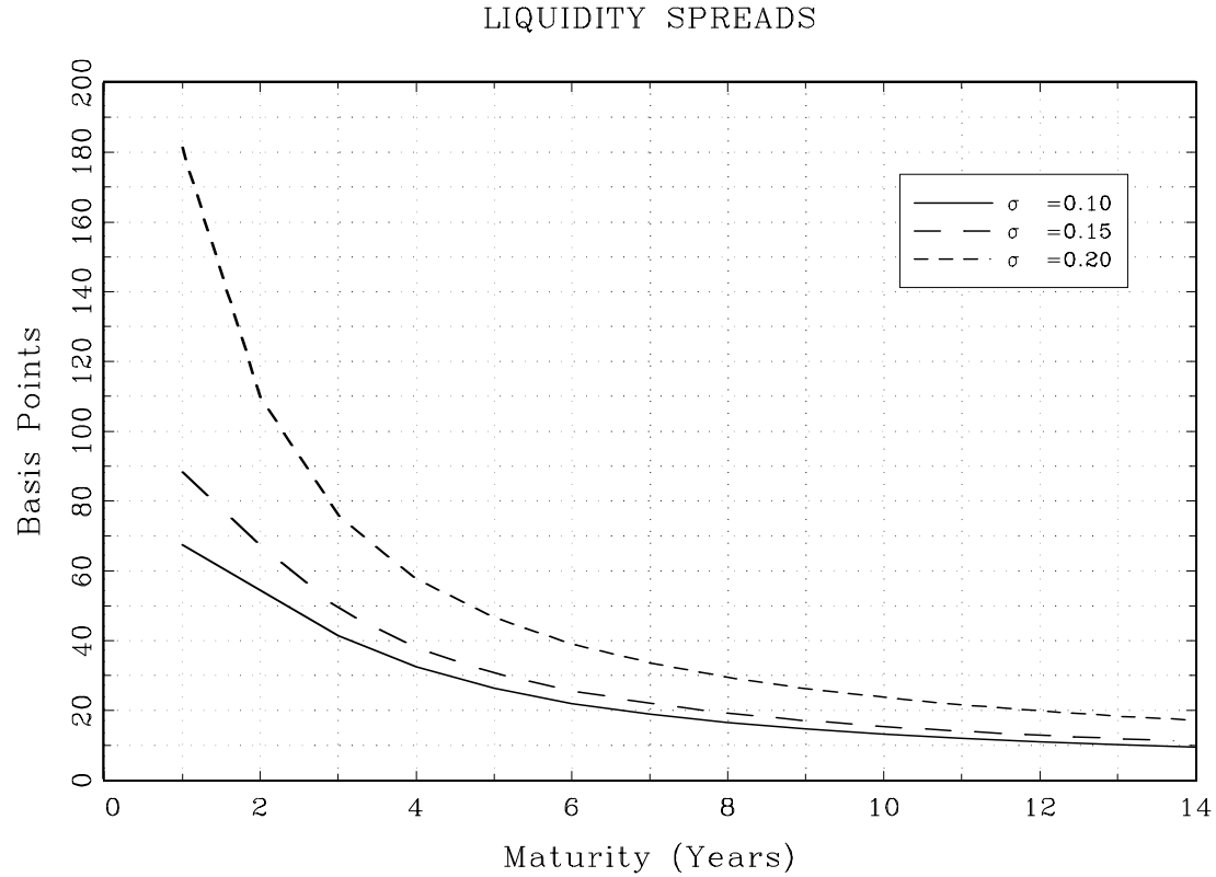
Figure 8: Liquidity spreads for varying levels of asset volatility. Other parameters : the time step is \Delta t = 1/12 (one month), the risk-free interest rate is r = 7\% , the average number of market-makers active for the security is \gamma = 7 , the probability of a liquidity shock is \theta = 0.427\% which corresponds to a yearly probability of 5% of having at least one shock and the quasi-debt ratio is q = 0.8 . The bankruptcy costs are K = 30 and the cost of illiquidit in the market for distressed debt is \kappa = 20 . The default threshold is set in proportion to the quasi debt ratio L = \exp(-rT)P .
