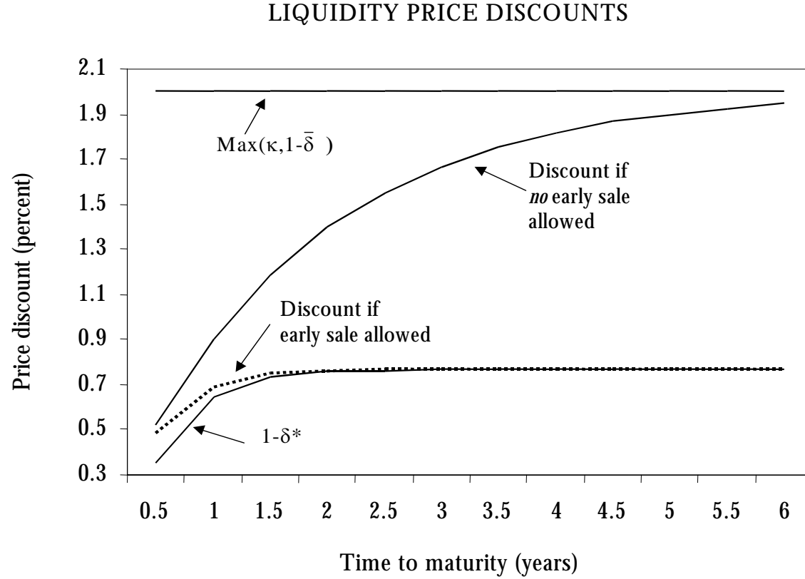
Figure 6: The price discount and its upper and lower bounds as functions of time to maturity. The upper bound corresponds to the worst case when the bondholder immediately enters into financial distress or is forced to sell. When there are no voluntary sales, the liquidity discount will eventually approach this upper bound as the probability of a forced sale approaches one. However, as this happens the likelihood of a voluntary sale increases, until the discount eventually approaches the lower bound corresponding to the reservation discount of the bondholder.
