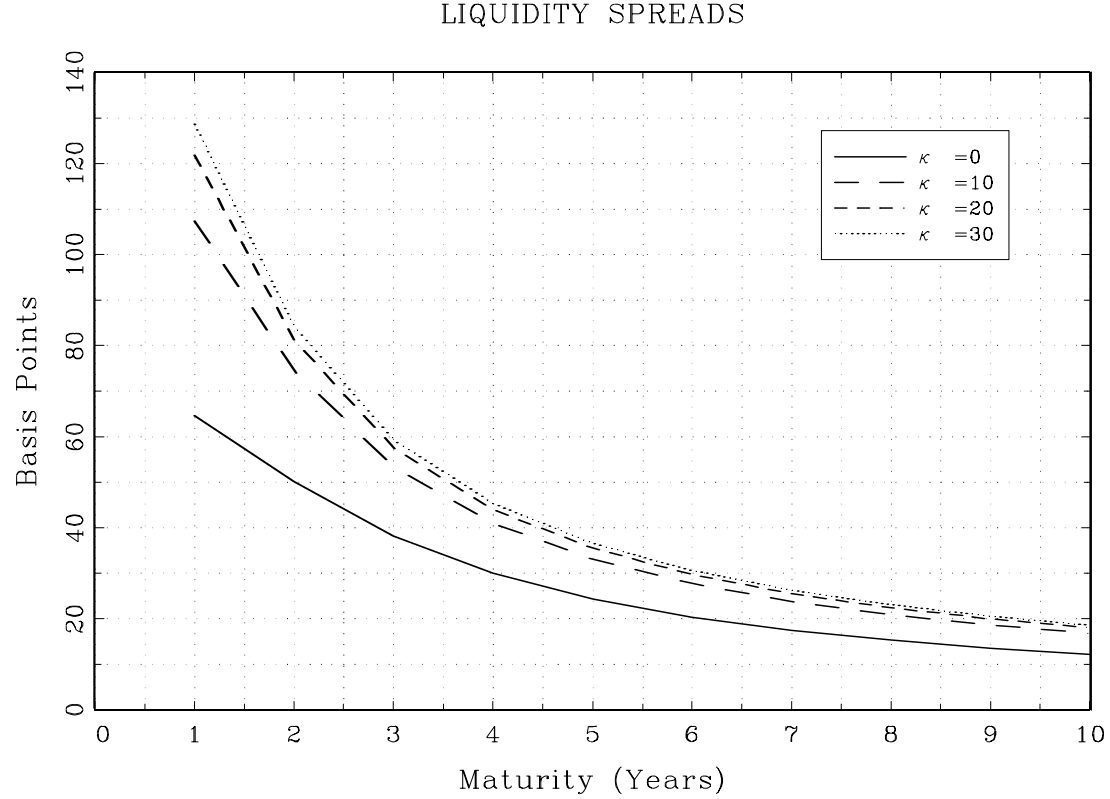
Figure 9: Liquidity spreads for varying levels of \kappa , the cost of illiquidity in the market for distressed debt. Other parameters : the time step is \Delta t = 1/12 (one month), the risk-free interest rate is r = 7\% , the average number of market-makers active for the security is \gamma = 7 , the probability of a liquidity shock is \theta = 0.427\% which corresponds to a yearly probability of 5% of having at least one shock and the quasi-debt ratio is q = 0.8 . The default risk related parameters are the asset volatility ( \sigma = 0.16 ), the bankruptcy costs K = 30 . The default threshold is set in proportion to the quasi debt ratio L = \exp(-rT)P .
