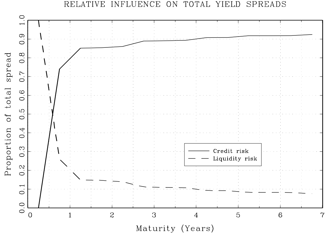
Figure 5: The percentage proportion of liquidity and credit risk compensation in the total yield spread. Parameters : the time step is \Delta t = 1/12 (one month), the risk-free interest rate is r = 7\% , the average number of market-makers active for the security is \gamma = 7 , the probability of a liquidity shock is \theta = 0.427\% which corresponds to a yearly probability of 5% of having at least one shock and the quasi-debt ratio is q = 0.8 .
