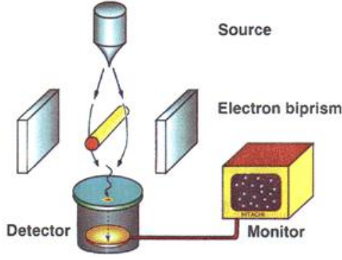
Figure 2: Experimental arrangement of a two-slit experiment with electrons. Two paths are made available to a weak electron beam via the electron biprism, a interferometric device composed of parallel plates with a fine central filament, the filament having a positive electrostatic potential relative to the plates. [Image courtesy of A. Tonomura, et al.: American Journal of Physics 57 (1989) 117-120.]
