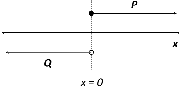
Figure 3: Phase space of a very simple classical system, that of a coin which can be heads or tails. Each potential property is associated with a subset of phase space, in this case the two halves of the real number line.
