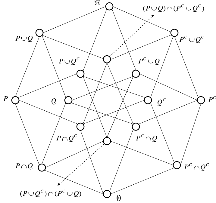
Figure 5: The graph of all possible subset relations involving the sets P, Q, P^C, Q^C . The lines indicate subset inclusion of the lower nodes by the higher nodes to which they are connected. This ‘lattice’ structure represents a simple Boolean algebra.
